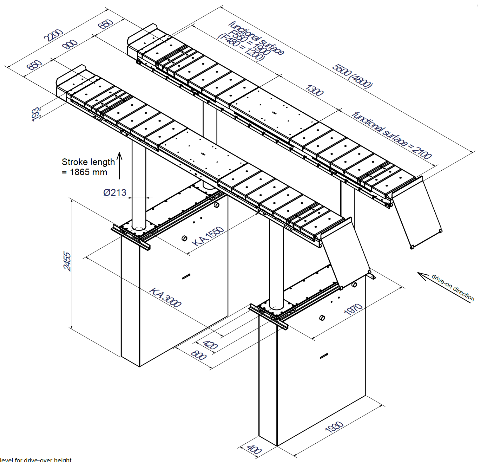
Dimension sketch incl. specifications of level for drive-over height.
