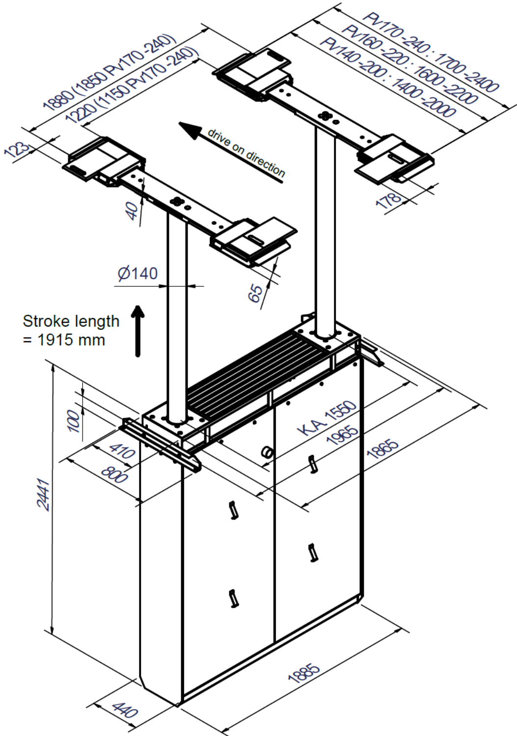
Dimensional sketch including drive-over heights
